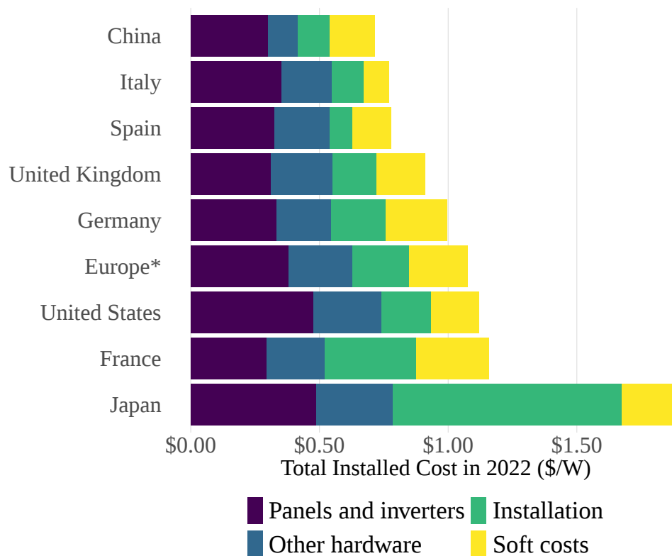
Figure A.1: Breakdown of utility-scale solar PV total installed costs by country in 2022
