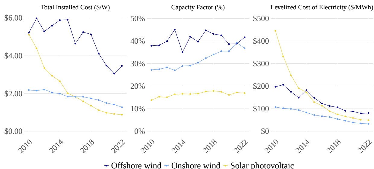
Figure 1: Trends in costs: total installed cost, capacity factor, and levelized cost of electricity
